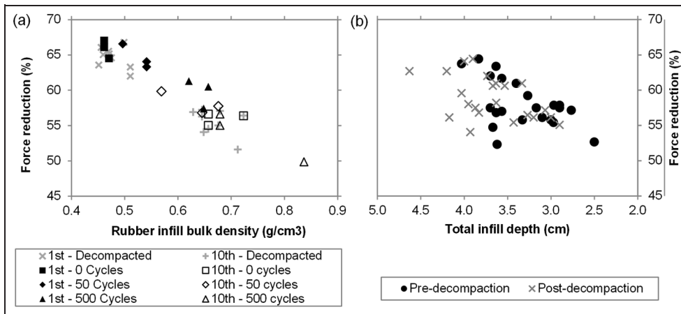
Figure 5. (a) Force reduction versus rubber infill net bulk density from laboratory testing. The data are from pre-1st impact and post-10th impact of the AAA immediately following the three levels of compactive effort and pre-1st impact and post-10th impact of the AAA immediately following the decompaction raking. (b) Force reduction versus total infill depth from the four field sites. The data are from pre-1st impact of the CT before (compacted, black) and after (decompacted, grey) the decompaction maintenance.
